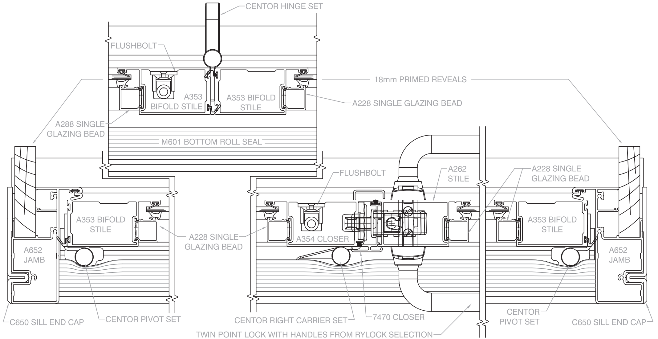
Scale 1 : 2 @ A4, Horizontal Cross Section of 3-Panel Bifold Door, >><
