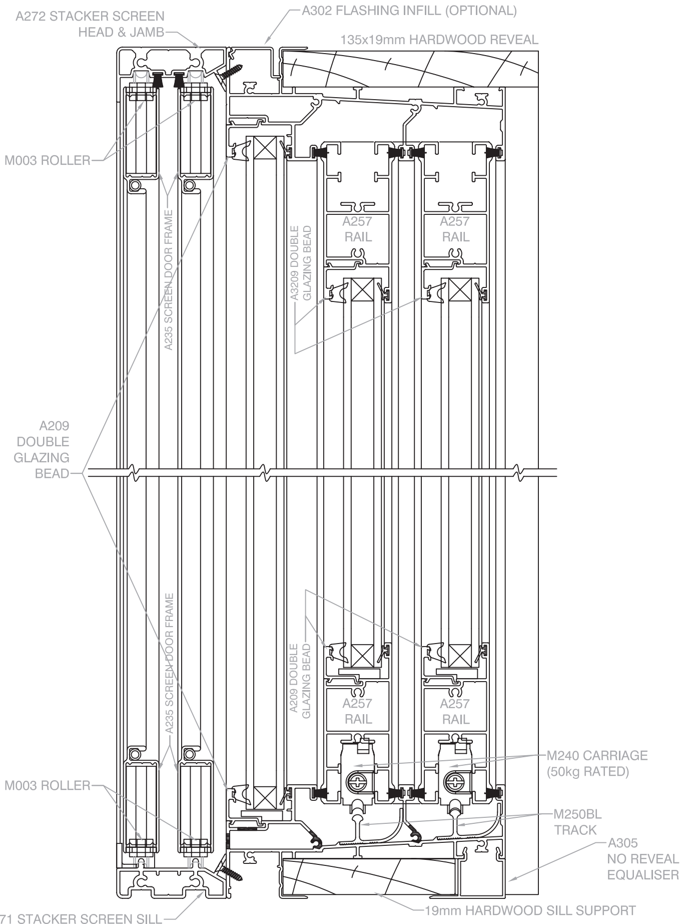
Scale 1 : 2 @ A4, Vertical Cross Section of 3 Panel - 3 Panel, Corner Stacker Door
